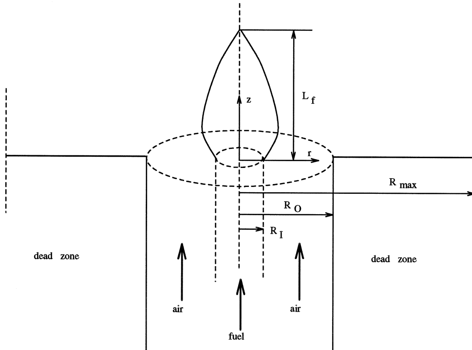
FIG. 1. Physical configuration (not in scale)
