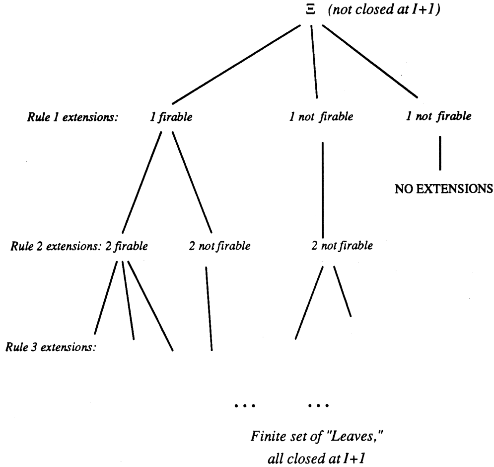
Figure 7: Tree of Extensions, "Leaves" Closed at I + 1
