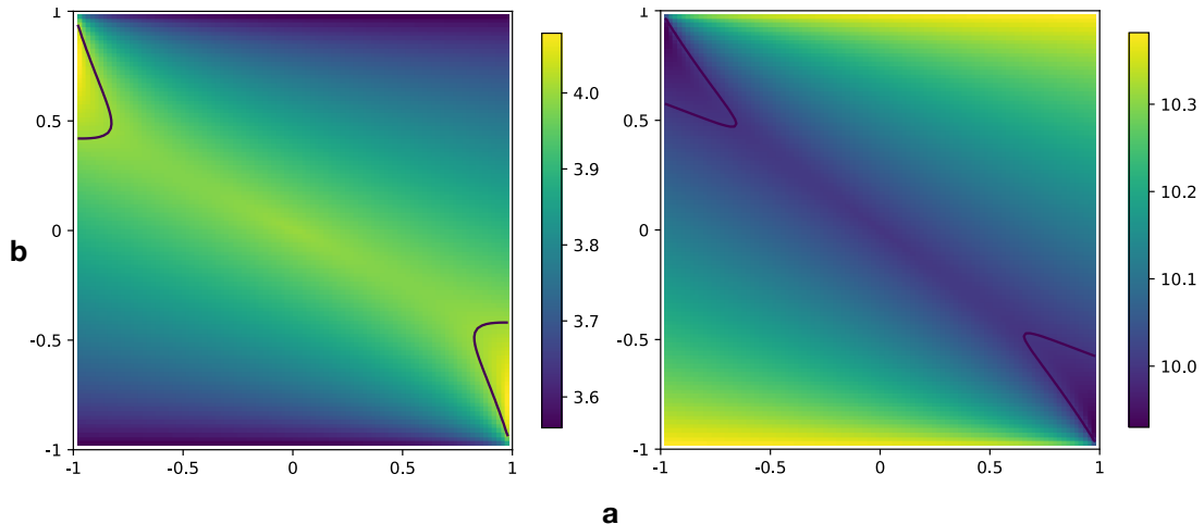
Figure 3: Plots for \beta(a, b) which satisfy \det \mathcal{A}_{\text{dir}}(a, b, \beta) = 0 at a triple junction with angles \theta_1 = \pi/\sqrt{2} , \theta_2 = \pi/\sqrt{3} . \beta(0, 0) = 4 for the figure on the left, and \beta(0, 0) = 10 for figure on the right. In both of the figures, the solid black lines indicate sections of the conjectured measure zero set S defined in conjecture 4.2.
