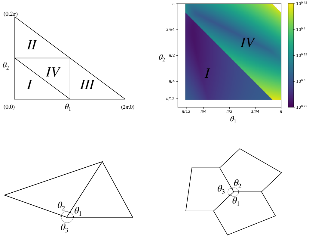
Figure 7: (top left) Regions I-IV in (\theta_1, \theta_2) simplex; (top right) condition number of discretized linear system corresponding to eq. (14) as a function of (\theta_1, \theta_2) ; (bottom left) sample domain for (\theta_1, \theta_2) in region I; (bottom right) sample domain for (\theta_1, \theta_2) in region IV.
