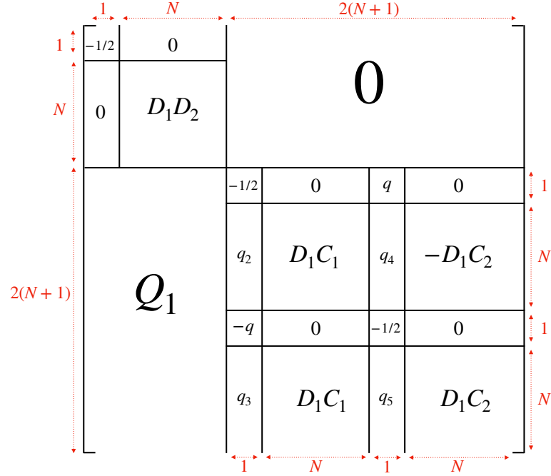
Figure 11: Structure of the matrix PBP^T
