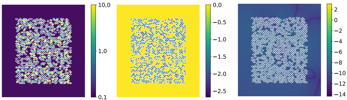
Figure 8: (left): Material parameters \nu_i for each of the regions, (center) exact solution u_j in the domains, and (right) \log_{10} of the absolute error in the solution. The geometry consists 3101 vertices, 3951 edges, 867 regions, and is discretized with 387314 points. In order for the solution of the linear system to converge to a residue of 10^{-15} , GMRES required 158 iterations for eq. (14), and 162 iterations for eq. (15) in the accuracy tests, and 153 and 156 iterations (for g_i = x_1 , and g_i = x_2 respectively) for eq. (15) in computing the polarization tensors.
