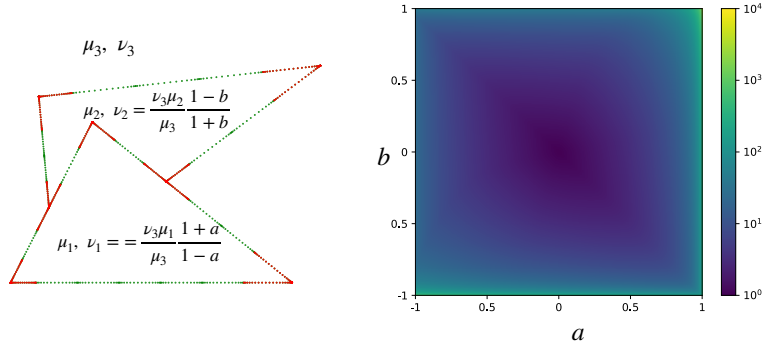
Figure 6: (left) Discretization of geometry and material parameters \mu, \nu as a function of a, b . Condition number as a function of (a, b) with \mu_1 = 0.37 , \mu_2 = 0.81 , \mu_3 = 1 , and \nu_3 = 0.77 .
