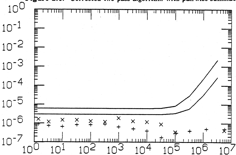
Figure 2.6. Corrected two-pass algorithm with pairwise summation
