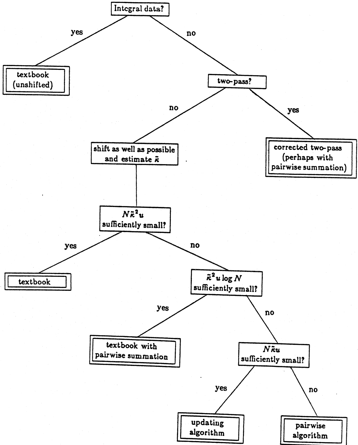
Figure 5.1. Decision procedure for choosing an algorithm to compute the variance. For details see the "Recommendations" section.
