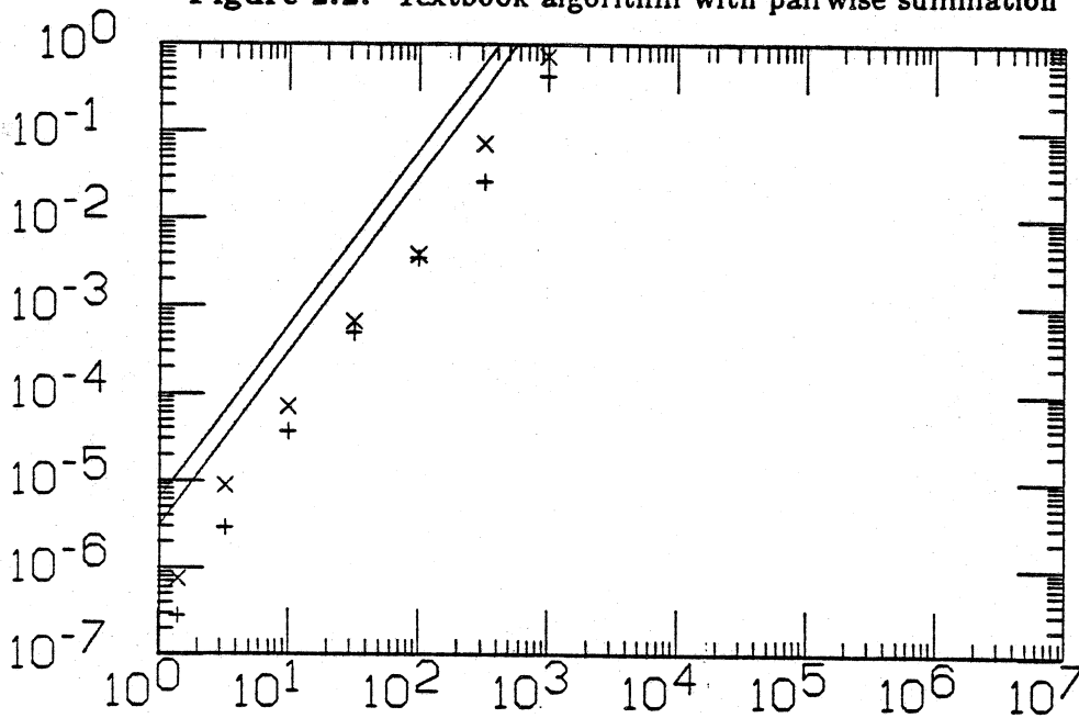
Figure 2.2. Textbook algorithm with pairwise summation
