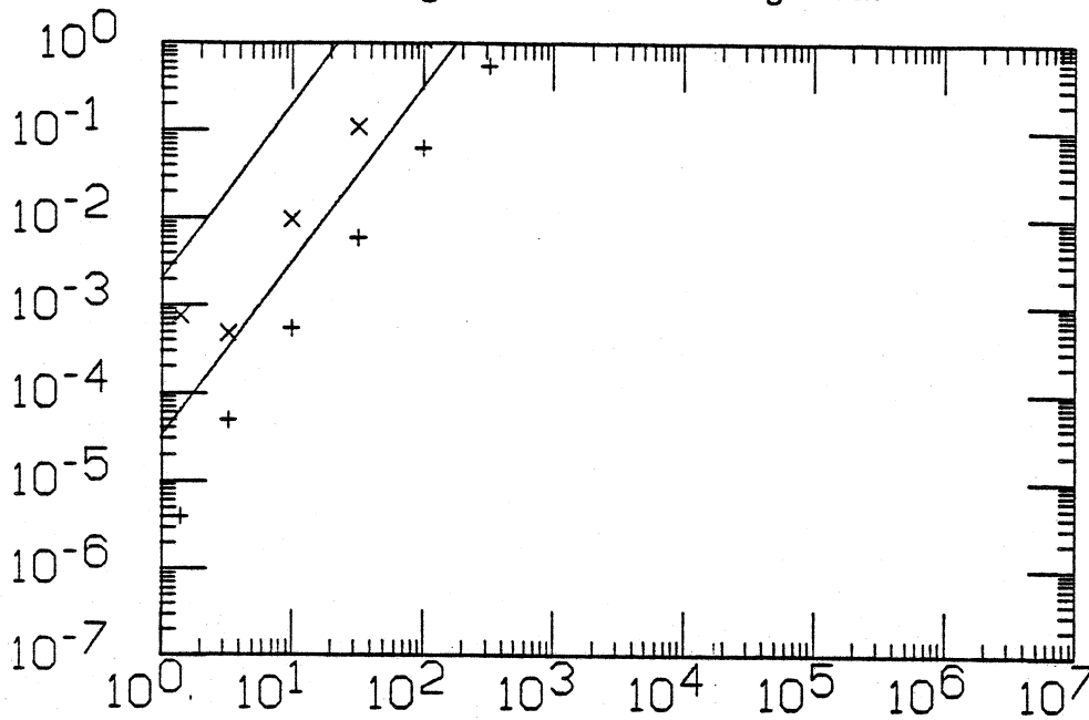
Figure 2.1. Textbook algorithm
