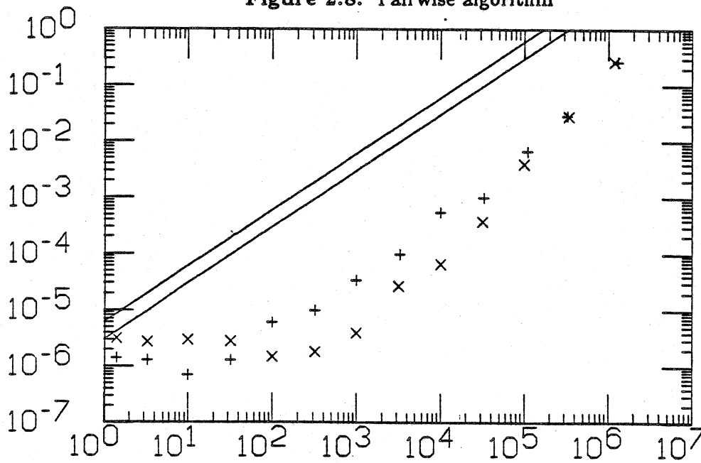
Figure 2.8. Pairwise algorithm
