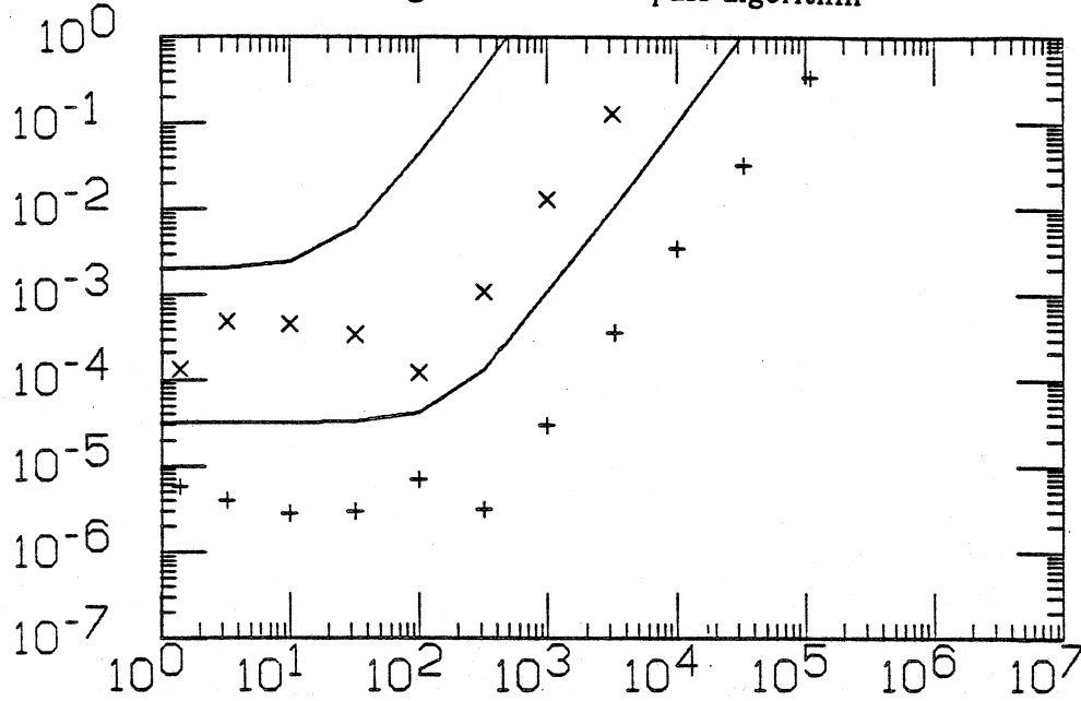
Figure 2.3. Two-pass algorithm
